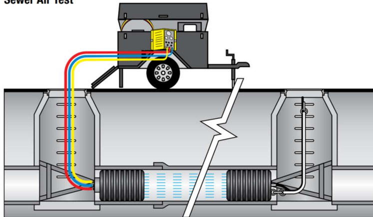
Sewer Air Test
